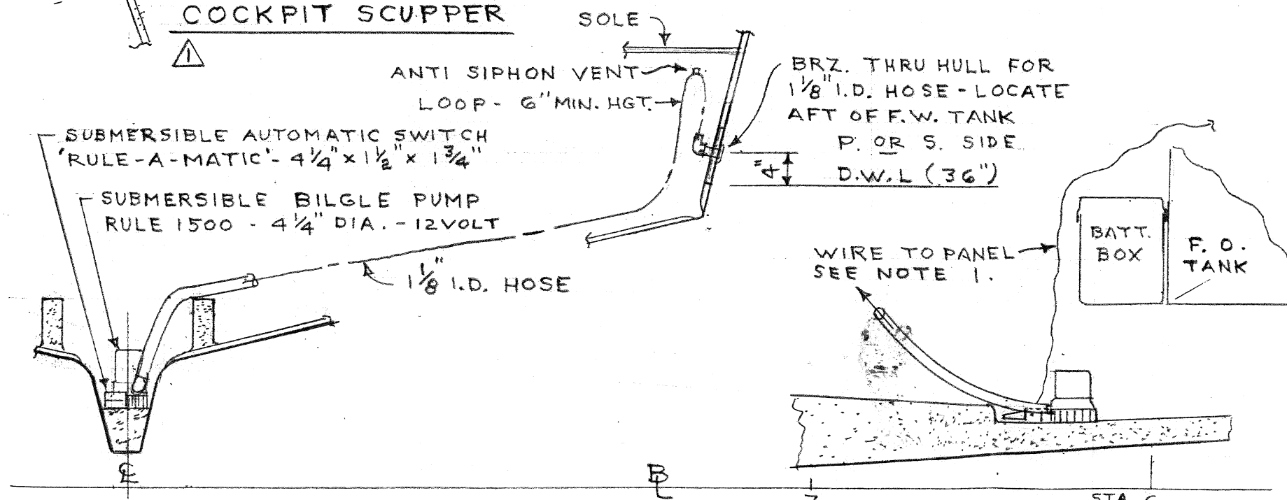
BILGE SYSTEM SECTION THRU SUMP
