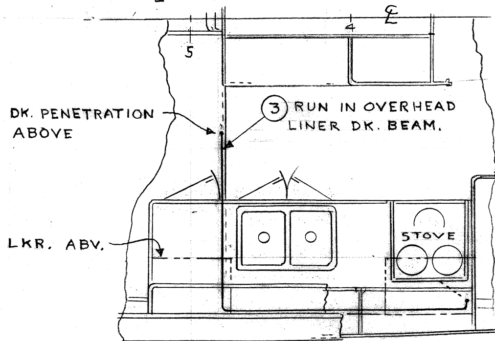
PLAN VIEW- FLY BRIDGE SCALE: 1/2" = 1'-0"
