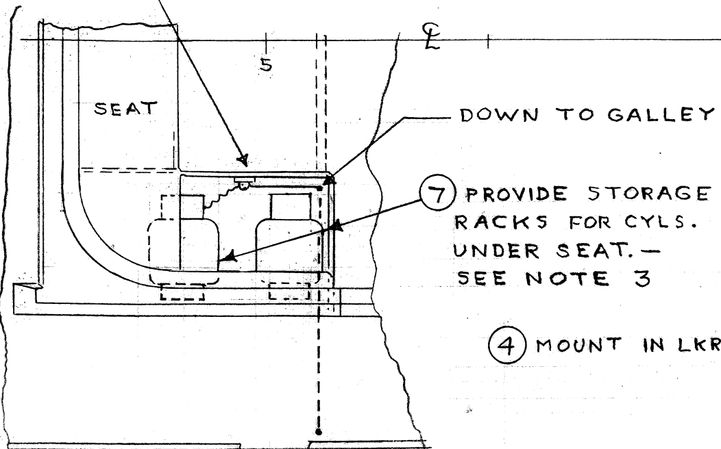
PLAN VIEW- FLY BRIDGE SCALE: 1/2" = 1'-0"
