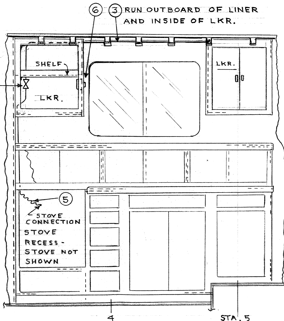
SECTION 3FT. OFF & LKG. TO STBD. GAS TUBE ROUTING IN GALLEY SCALE: 3/4" = 1'-0"
